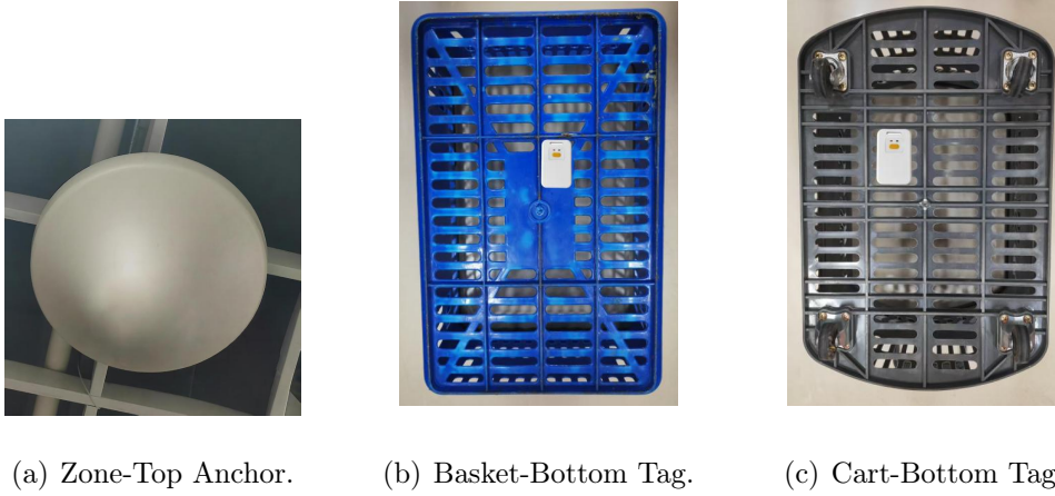
Figure 2: Experimental Equipment.
